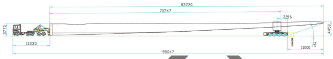
Figure 2: An indicative illustration of the blade transportation. 2
